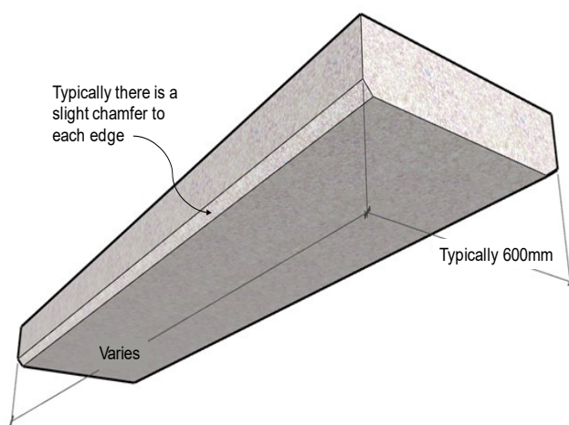
Figure 88: Profile of RAAC panels
